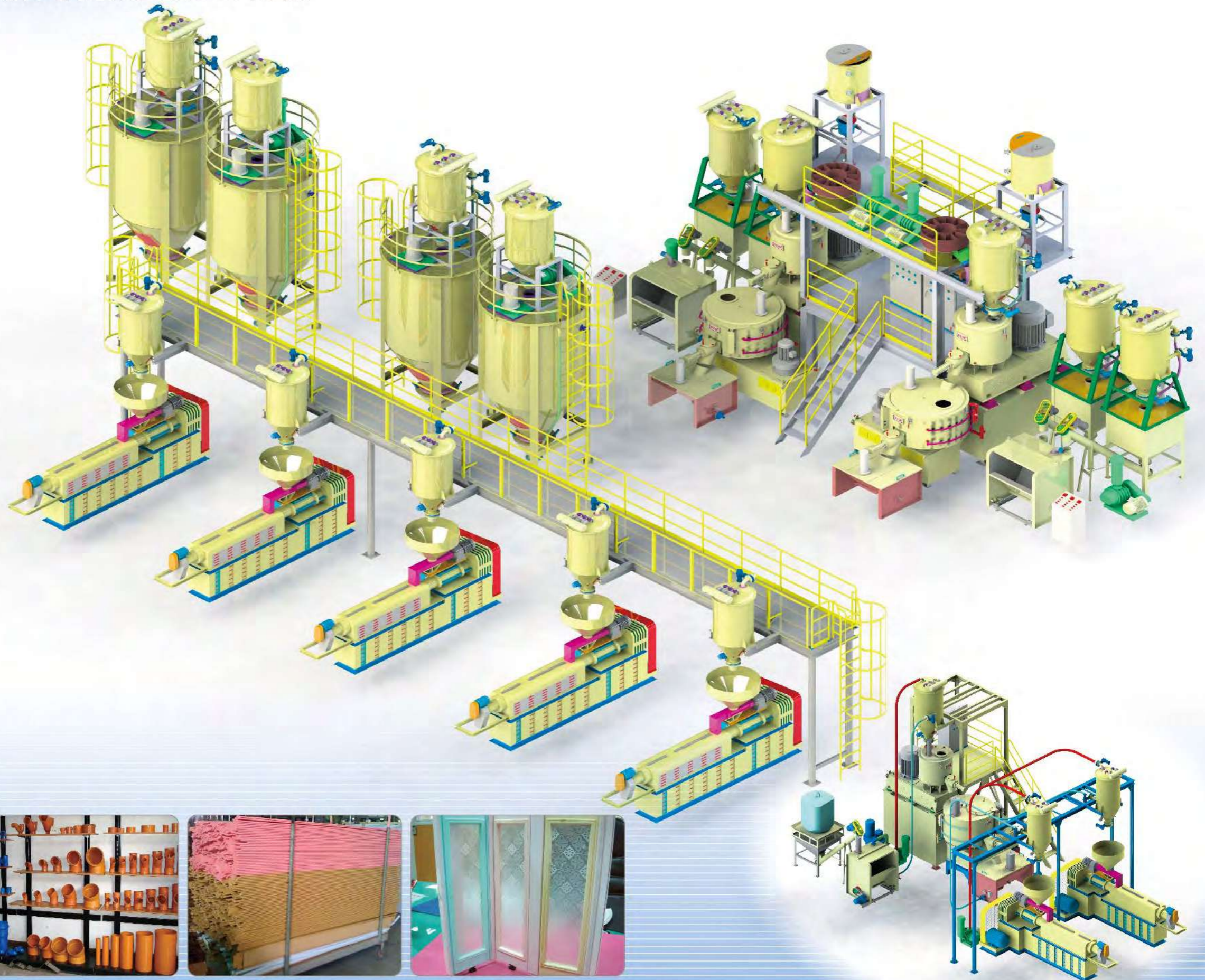
▲ PVC管&管件 PVC PIPE & FITTING
