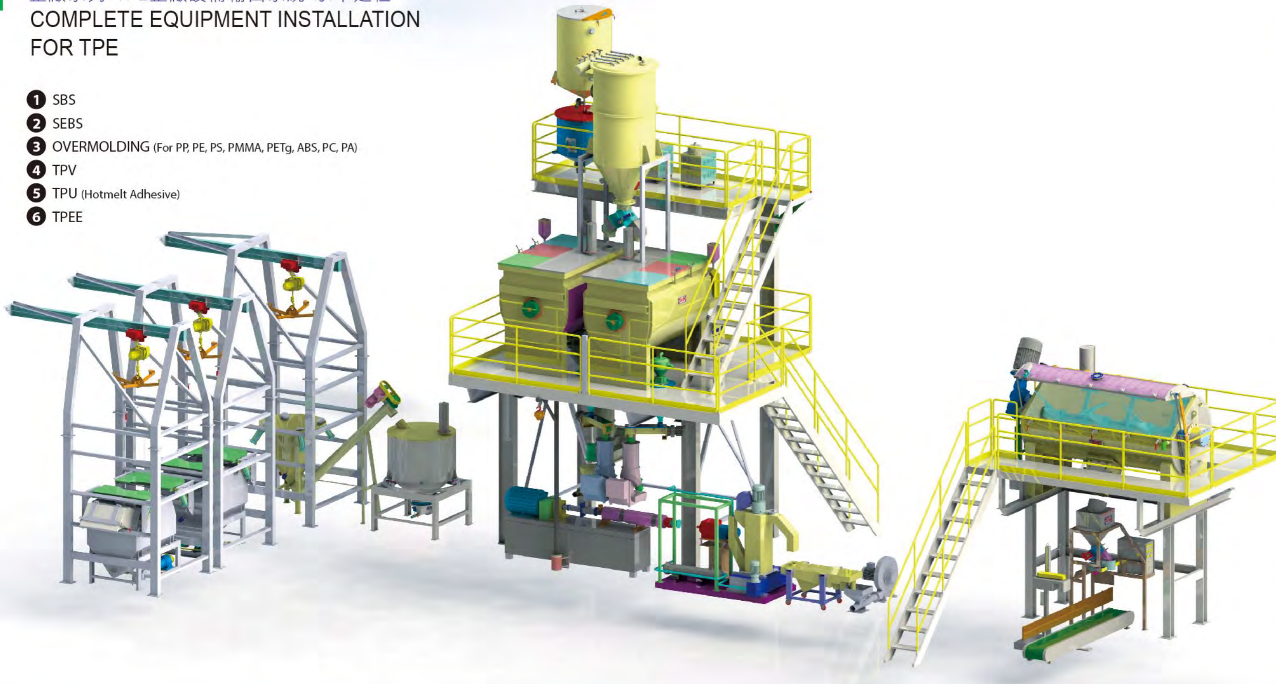
▲ TPE整廠設備 COMPLETE EQUIPMENT FOR TPE
