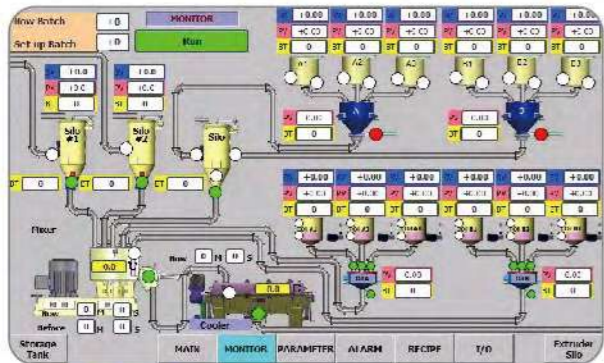
▲ 人機觸控螢幕介面 HMI TOUCH PANEL CONTROL SYSTEM
