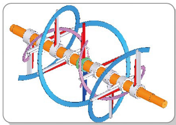
▲ 雙帶攪拌軸組 DOUBLE RIBBON MIXING BLADE
