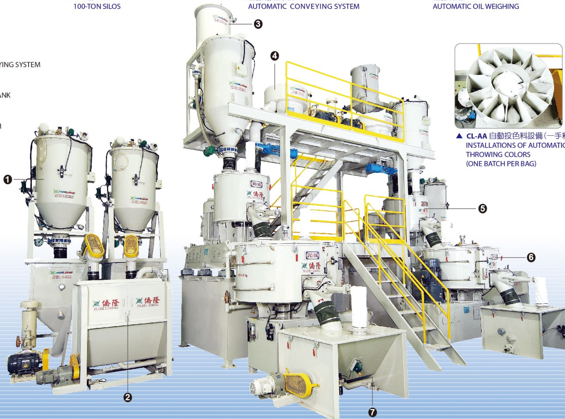
3 自動秤油系統 AUTOMATIC OIL SCALING SYSTEM
