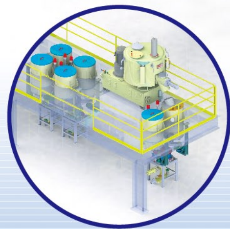
▲ 小量計量 (綜合安定劑、耐寒、耐熱、 抗氧化劑、DOP...等) SMALL QUANTITY ADDITIVES WEIGHING (PREMIXED STABILIZERS, ANTIOXIDANTS, IMPACT MODIFIERS, ETC.)
